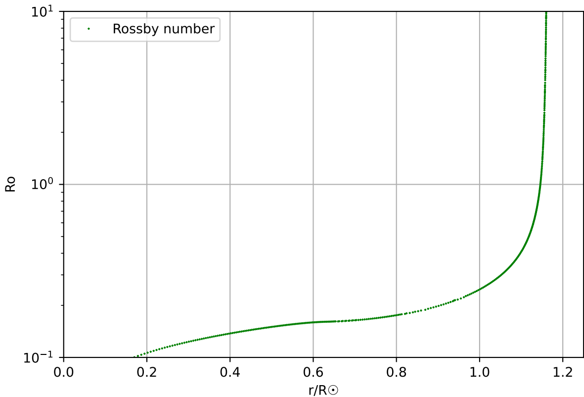
Rossby number, profile 104, age 1.27 \times 10^7
